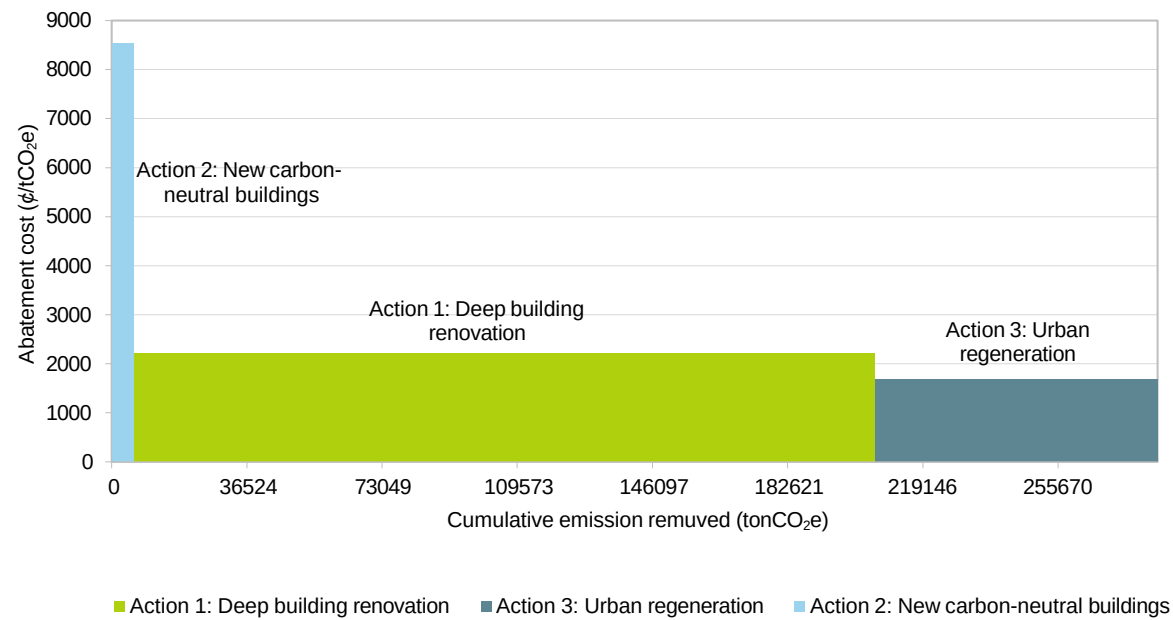
Figure 30. GHG emission abatement curve for the proposed actions
