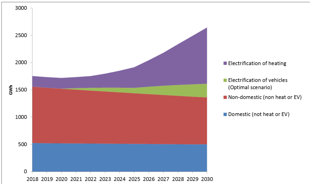
Figure 9: Forecast electricity demand for Bristol 2018-30 with heat and vehicle electrification
